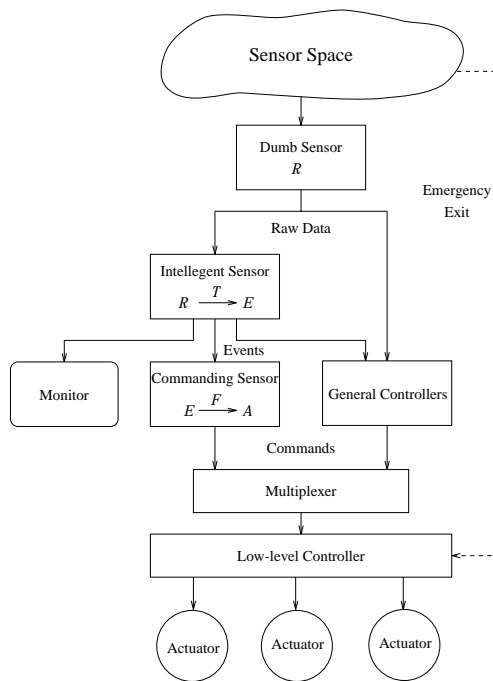
Figure 3: The proposed control scheme.
